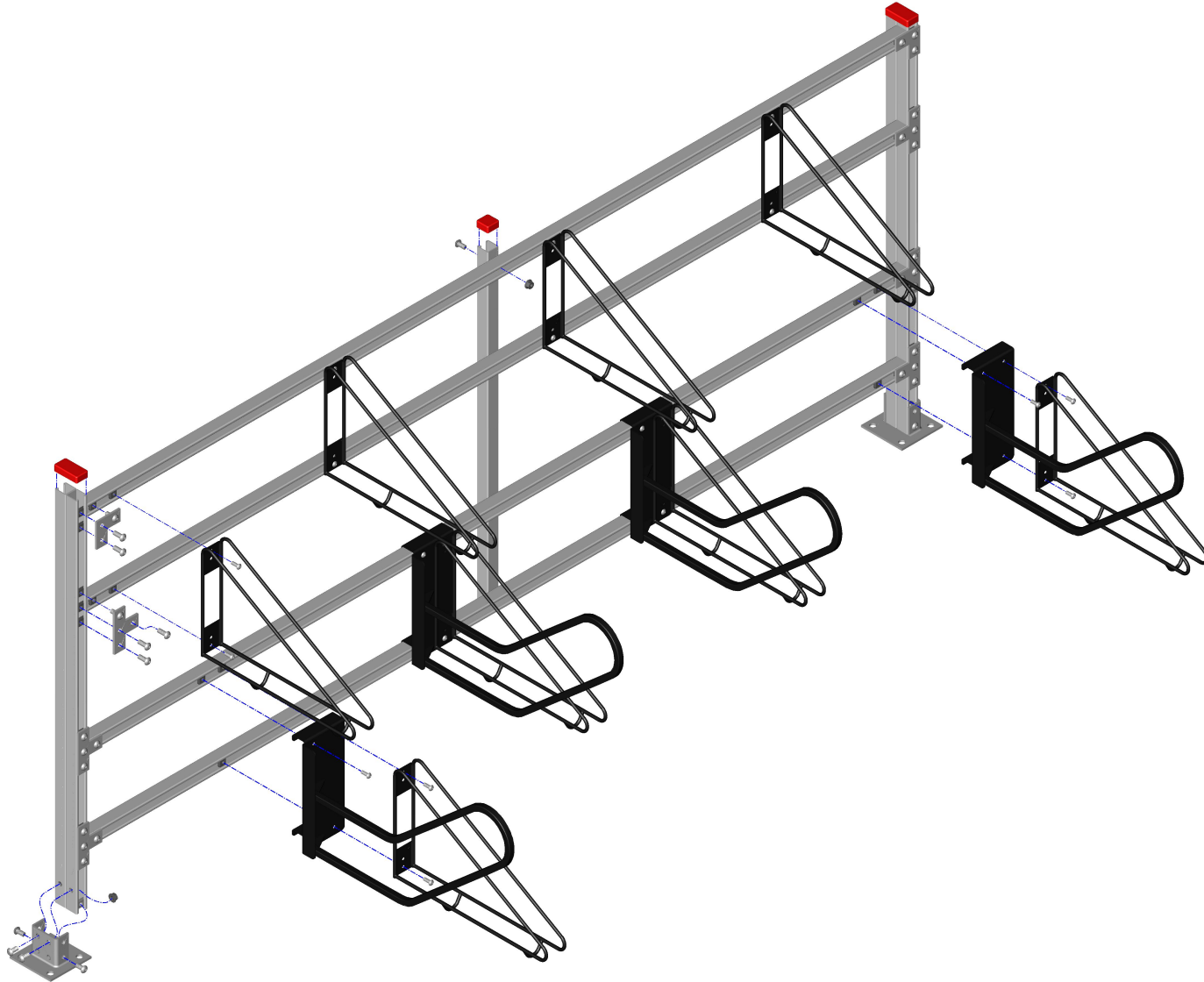
Bike Stall {8-Bike} H-Strut Post Base {Hi-Lo} Assembly {Exploded}
